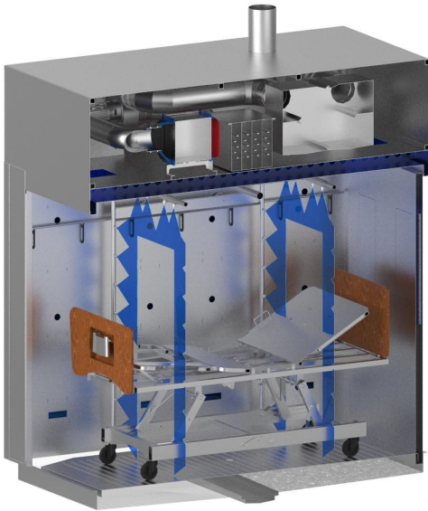
INSIDE VIEW OF CABINET WASHER-DISINFECTOR
